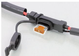
Fuse box includes 5A low-profile fuse.
